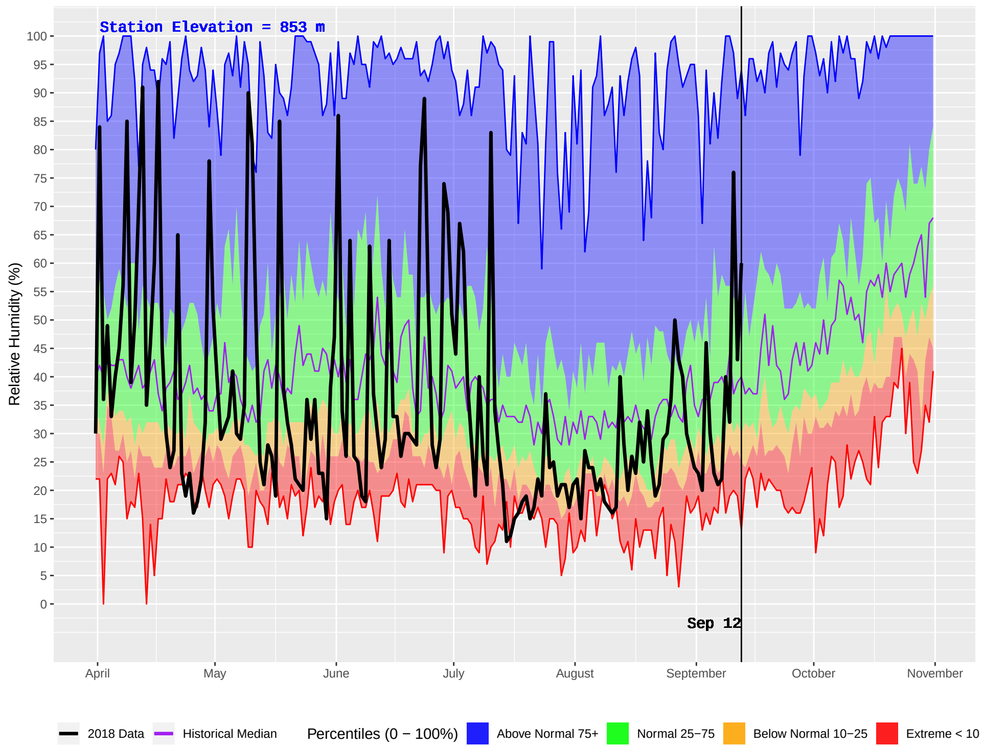
JOHNSON LAKE (419) : Historical (1986–2016) and Current (2018) Daily Relative Humidity
