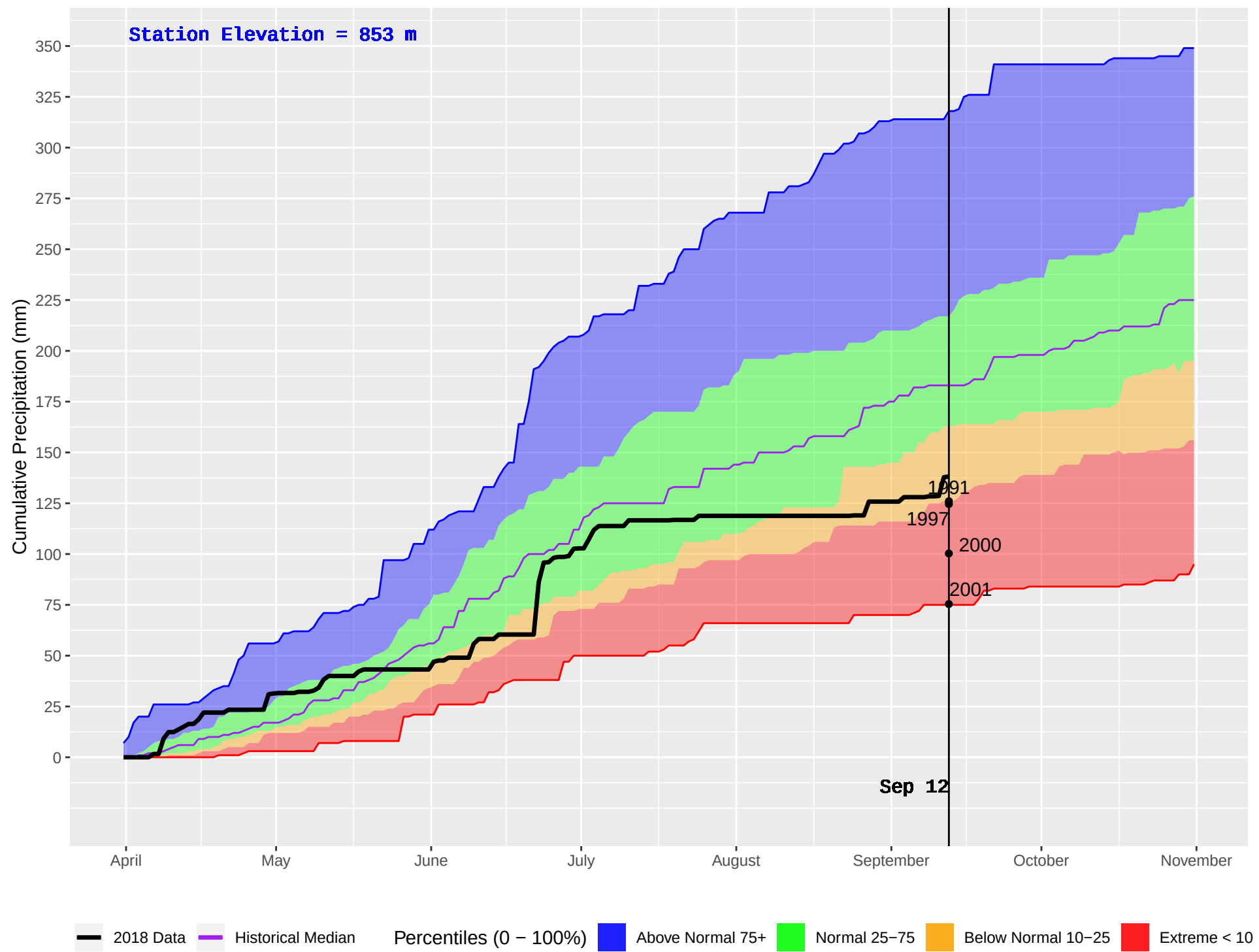
JOHNSON LAKE (419) : Historical (1986–2016) and Current (2018) Daily Cumulative Precipitation
