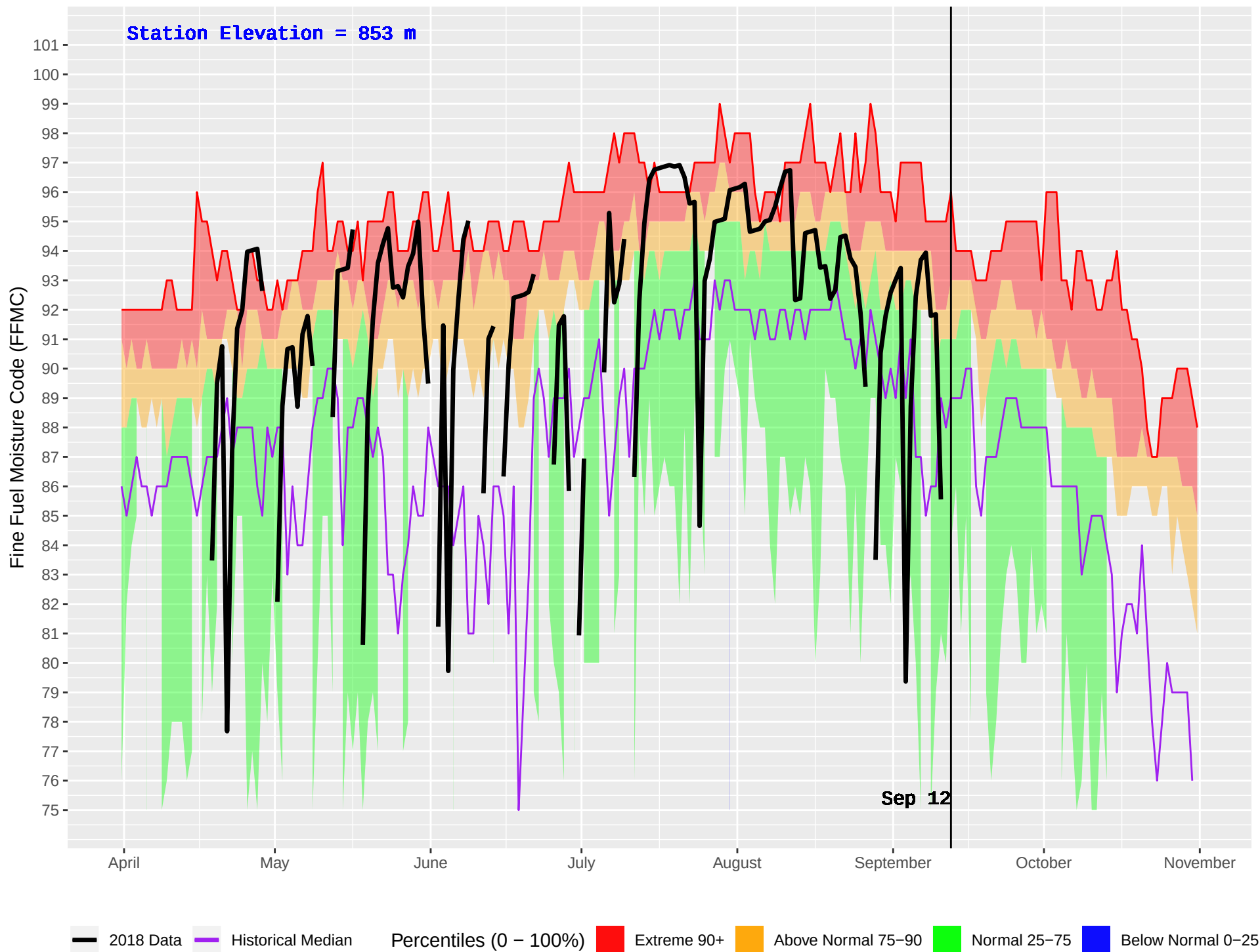
JOHNSON LAKE (419) : Historical (1986–2016) and Current (2018) Daily Fine Fuel Moisture Code (FFMC)
